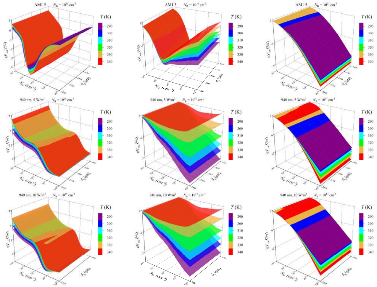
Fig.S3.11. Relative changes in open-circuit voltage caused by a complete dissociation of \text{Fe}_i\text{B}_s pairs as a function of iron concentration and base depth for different temperatures. N_B , \text{cm}^{-3} : 10^{15} (left panels), 10^{16} (middle panels), 10^{17} (right panels).
