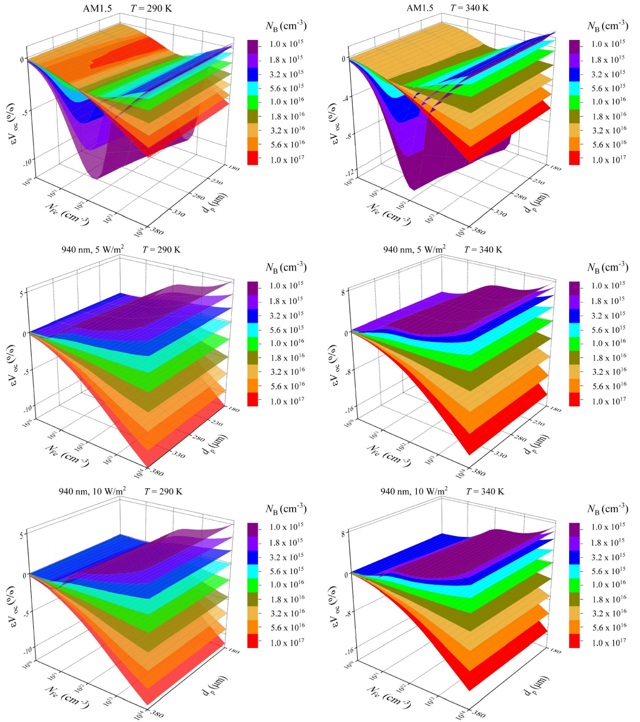
Fig.S3.12. Relative changes in open-circuit voltage caused by a complete dissociation of Fe_iB_s pairs as a function of iron concentration and base depth for SC with different base doping level. T, K: 290 (left panels), 340 (right panels).
